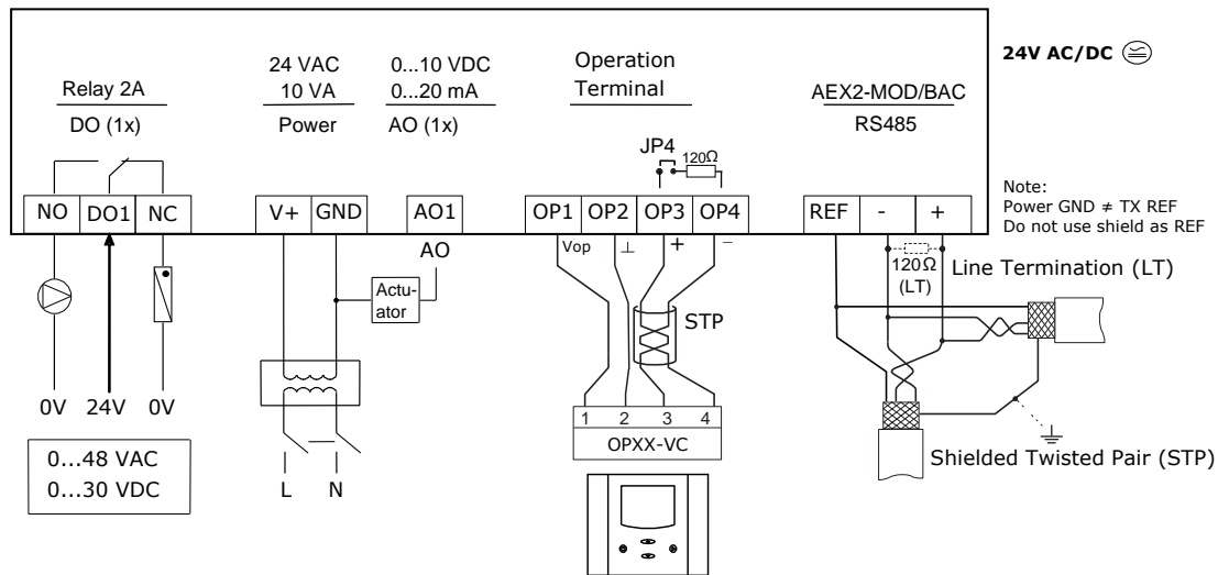
Connection diagram SDC2-200
