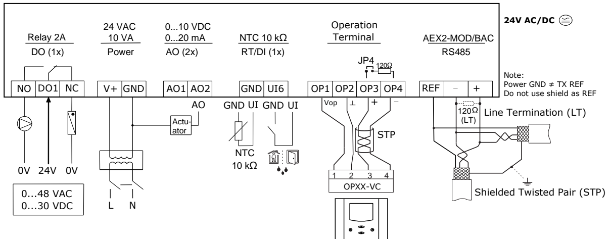
Connection diagram SDC2-210
