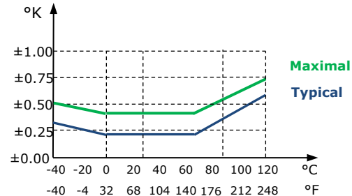
Figure 2: Typical and maximal temperature accuracy
